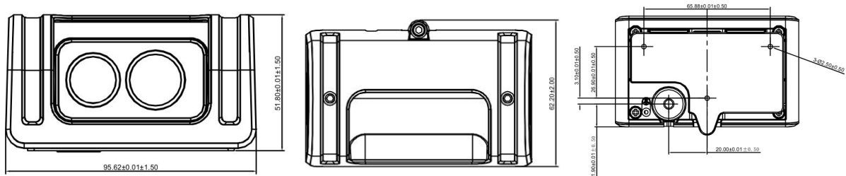
Product size diagram
