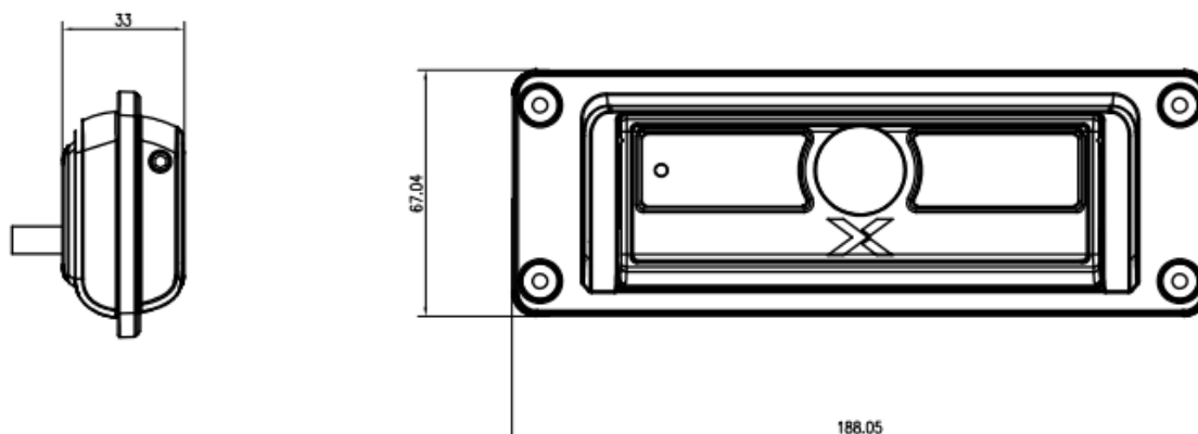
Built-in installation method (mm)
