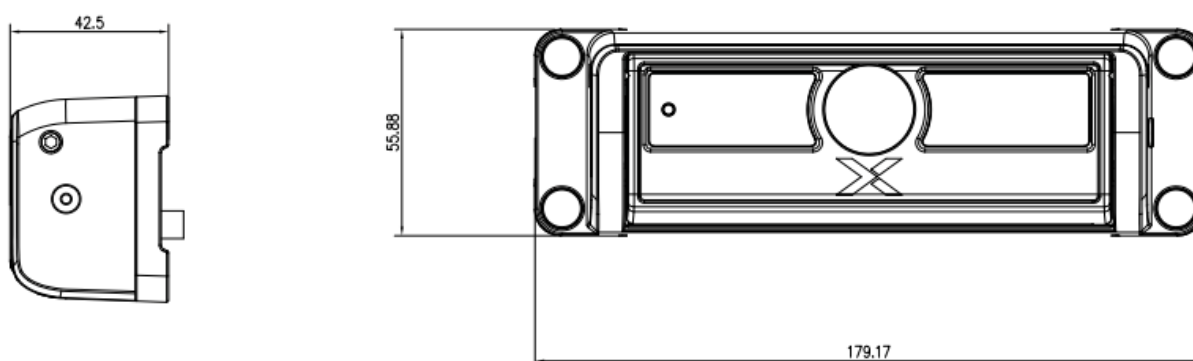
Side installation method (mm)
